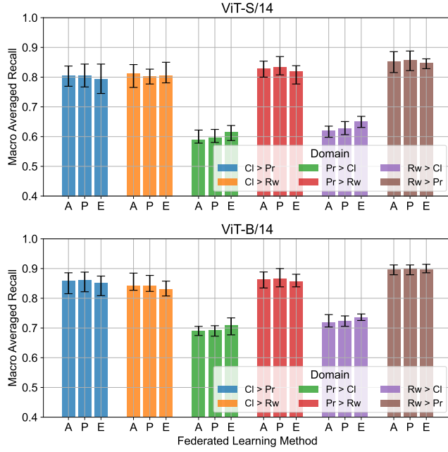
Fig. 6: The comparison among three different federated learning method, FedAvg (A), FedProx (P), and FedETF (E), with OH. Note that in this figure, colors indicate different source-target pairs. Each plot shows the average over nine runs, comprised of three different source imbalance ratios and three different target imbalance ratio. Error bars represent the maximum and minimum values from these nine runs.
