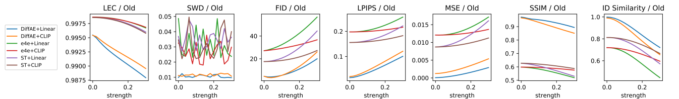
Fig. 2. Evaluation results for the “old” attribute under different editing strengths.
