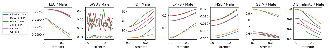
Fig. 3. Evaluation results for the “male” attribute under different editing strengths.
