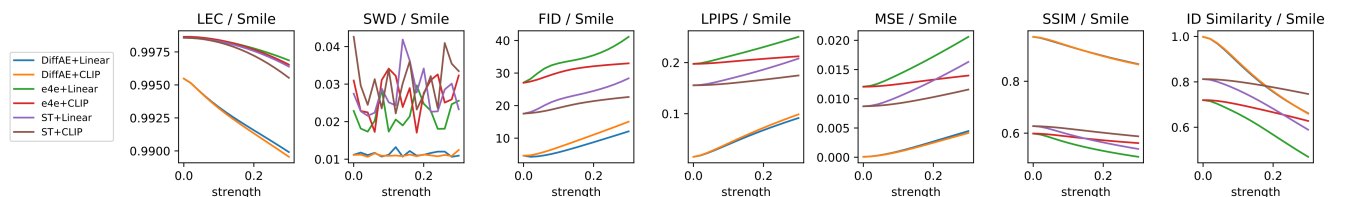
Fig. 4. Evaluation results for the “smile” attribute under different editing strengths.
