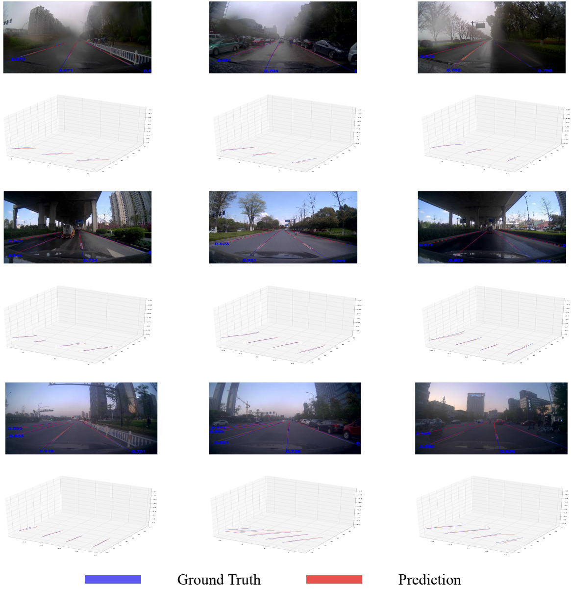
Fig. 2: Qualitative results on the ONCE-3DLanes dataset.
