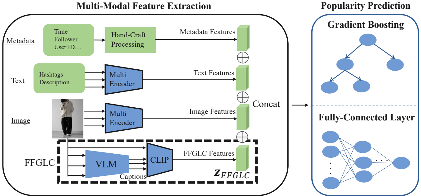
Fig. 2. Overview of the popularity prediction framework proposed in [3, 4, 5]. Features are extracted from metadata, text, and images, and the integrated features are used to predict popularity scores using gradient boosting or fully-connected layers. Metadata consists of numerical and categorical features, which are appropriately preprocessed. For text and images, features are extracted using pre-trained multi-encoders. Specifically, text features are extracted using models such as BERT or FastText, while image features are extracted using models such as ResNet or CLIP. Additionally, integrating FFGLC features with these extracted features enhances the accuracy of popularity prediction. Since feature extraction and popularity prediction are separate processes, we train the models enclosed in blue boxes to perform popularity prediction using the extracted features.
